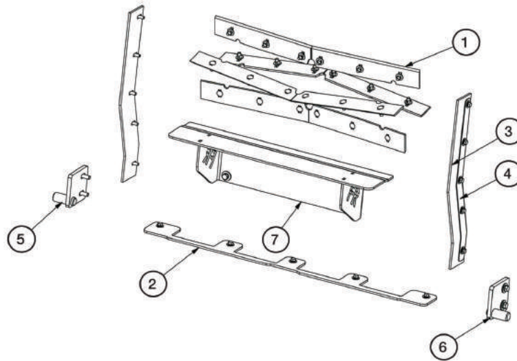
KFR9000 Kit
