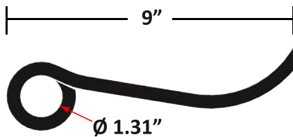
Part # K5200012
