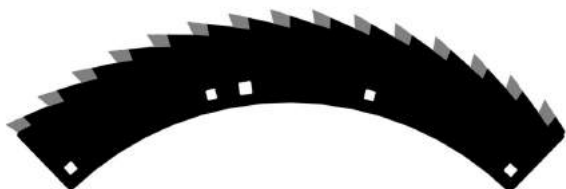
KK67746LTC – $36.50 ea. 2 lbs. To fit: JD® 684 4-row, 686 6-row, 688 8-row, 710 10-row To fit: Kemper™ 330 4-row, 345 6-row, 360 and 6008 8-row, 375 10-row
